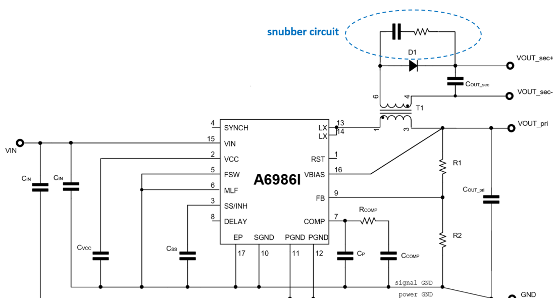
Figure 47. Snubber circuit
