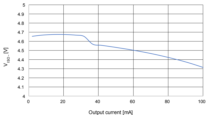
Figure 61. STEVAL-A6986IV1, V_{IN} = 12\text{ V} , f_{SW} = 500\text{ kHz}
