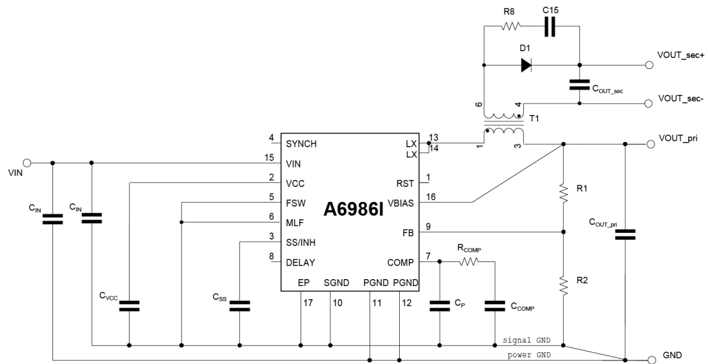
Figure 1. Application schematic
