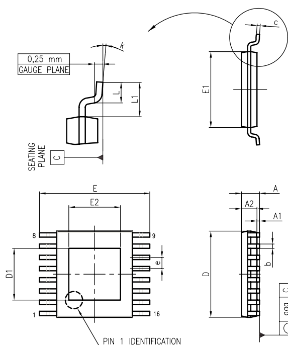
Figure 67. HTSSOP16 package outline
