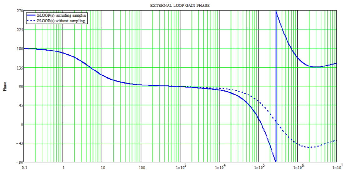
Figure 30. Bode plot (phase)
