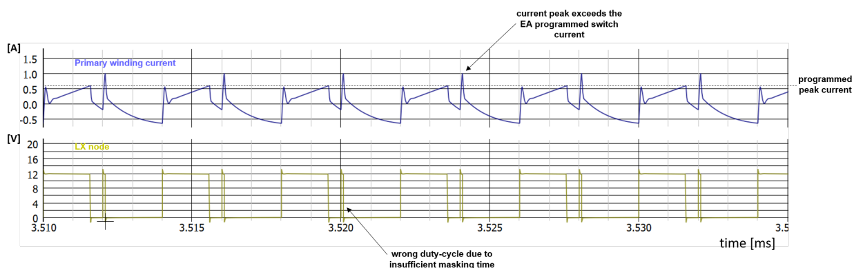
Figure 12. Simulation with insufficient masking time (< 100 ns)
