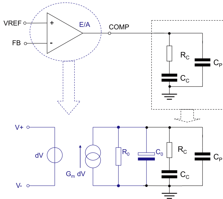
Figure 27. Transconductance embedded error amplifier
