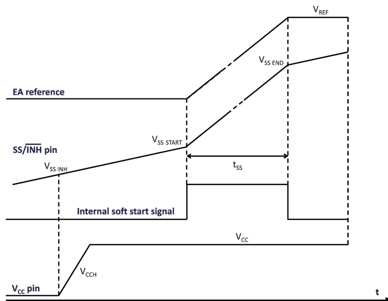
Figure 9. Soft-start phase
