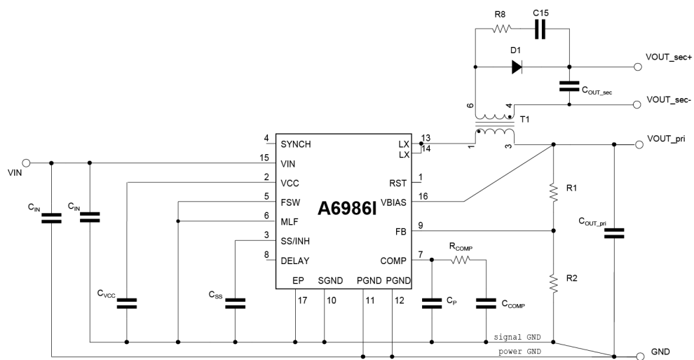
Figure 31. A6986I application circuit
