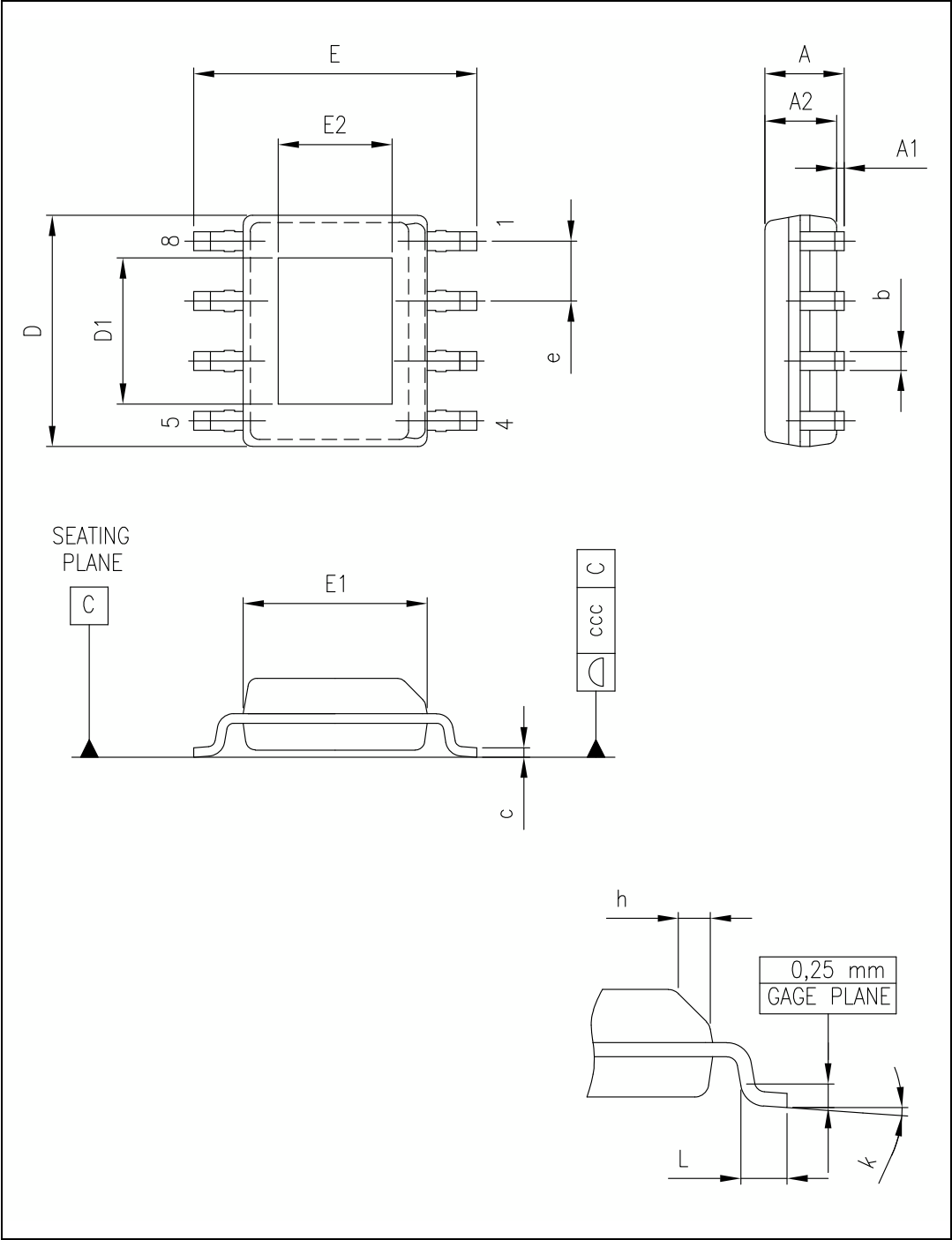
Figure 42. Package dimensions
