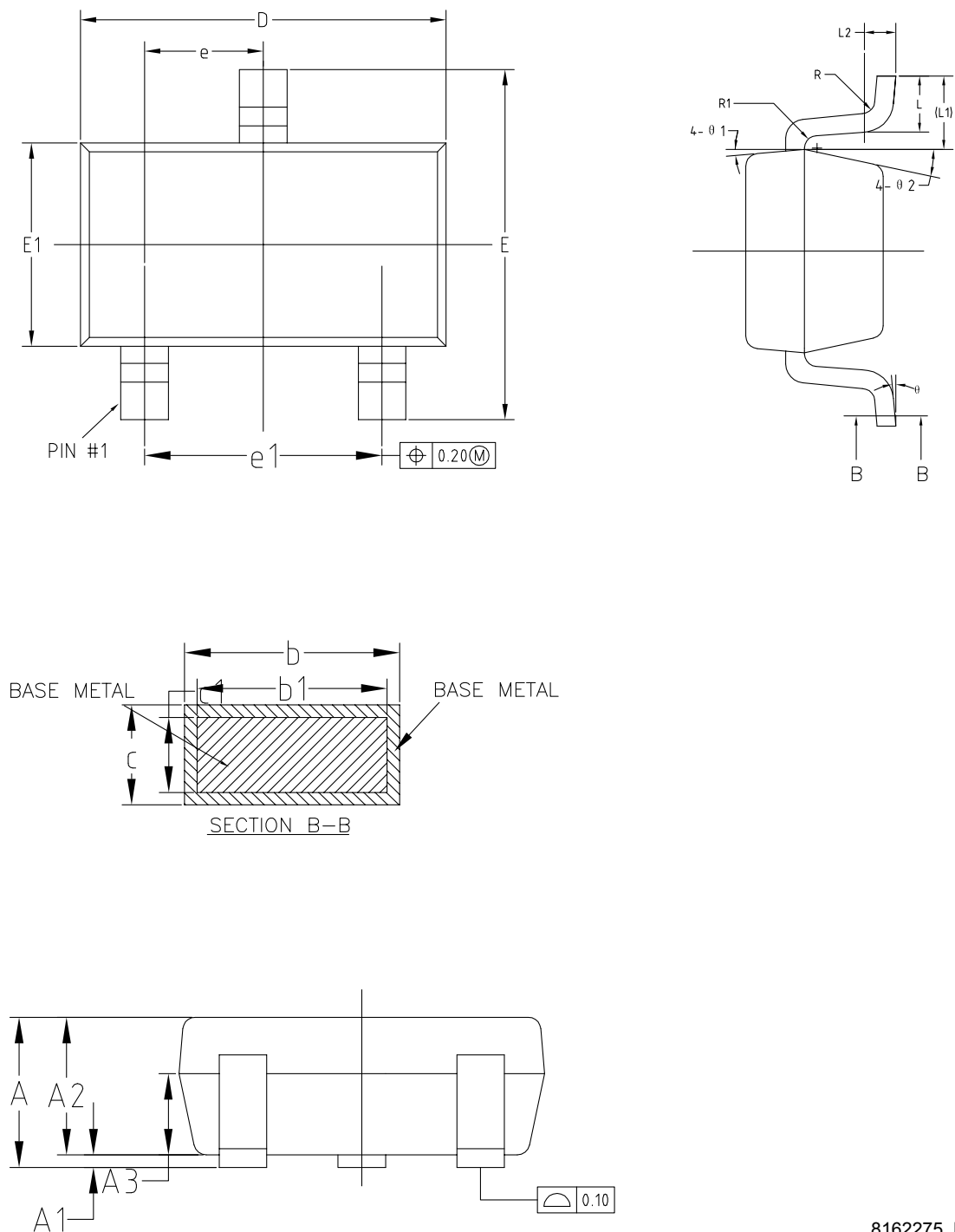
Figure 9. SOT-23 package outline (dimensions are in mm)
