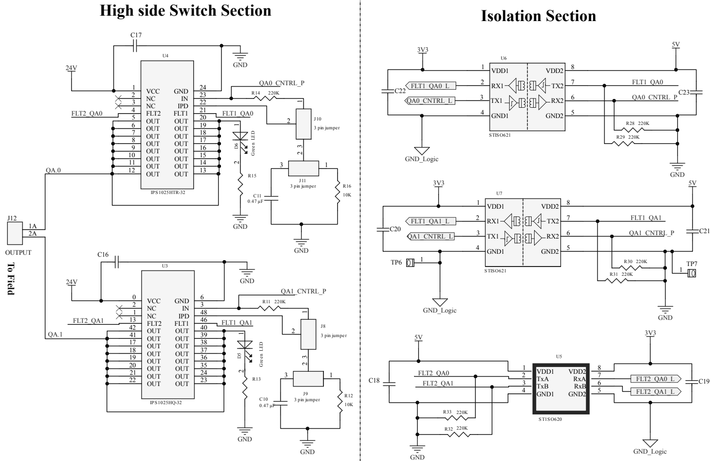
Figure 3. X-NUCLEO-ISO1A1 circuit schematic (3 of 4)
