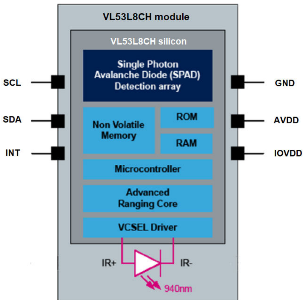
Figure 1. VL53L8CH block diagram
