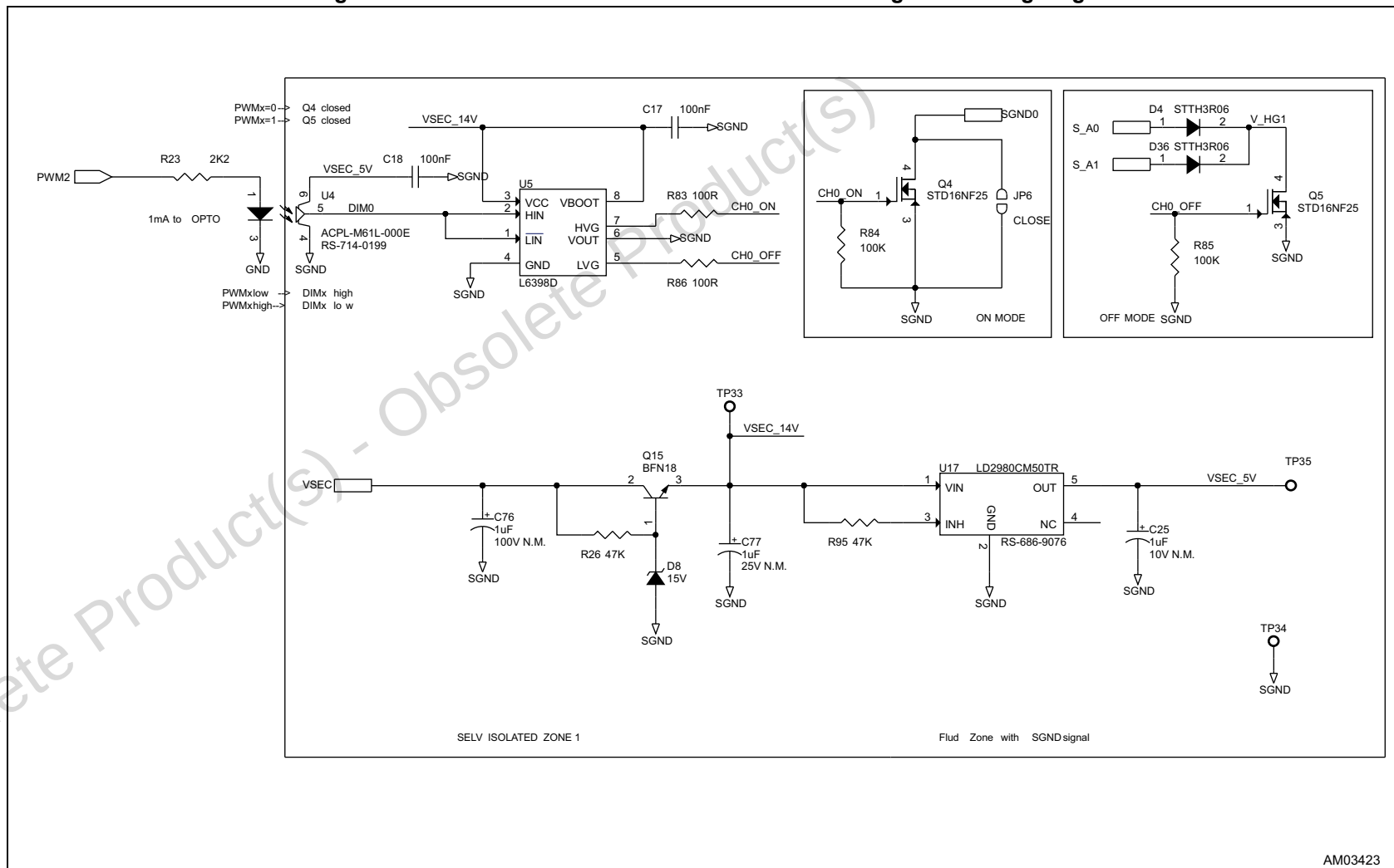
Figure 5. PSR-ZVS demonstration board schematic - digital dimming stage
