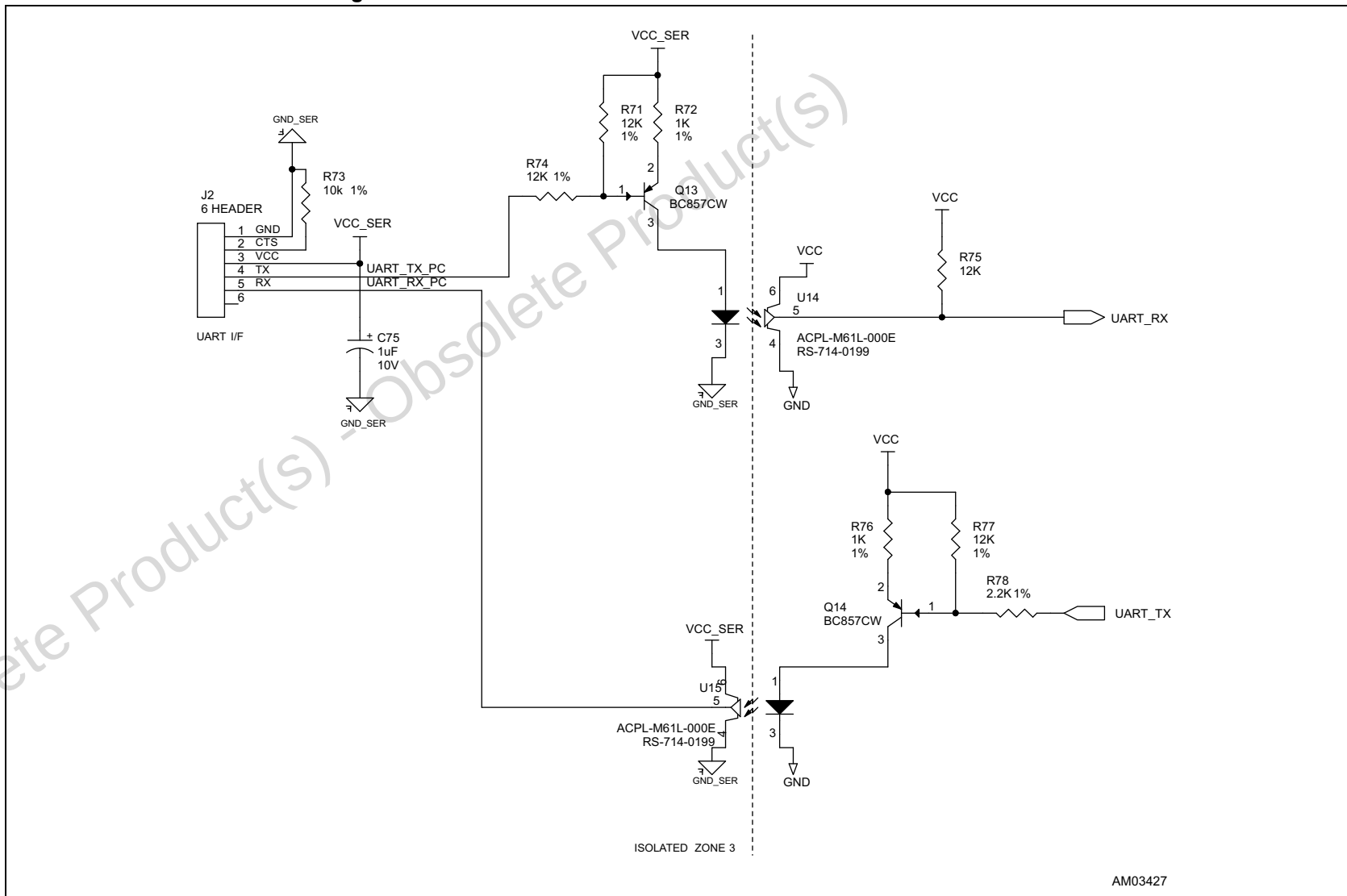
Figure 8. PSR-ZVS demonstration board schematic - serial interfaces
