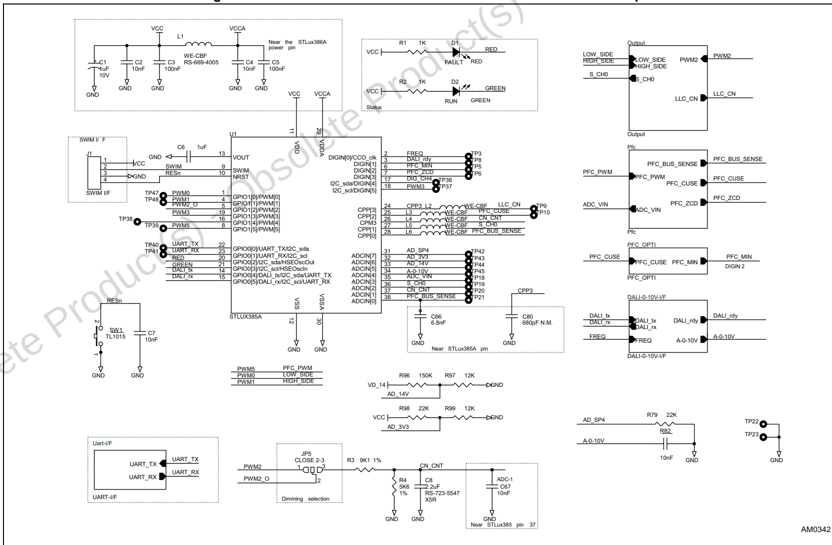
Figure 2. PSR-ZVS demonstration board schematic - STLUX385A - top
