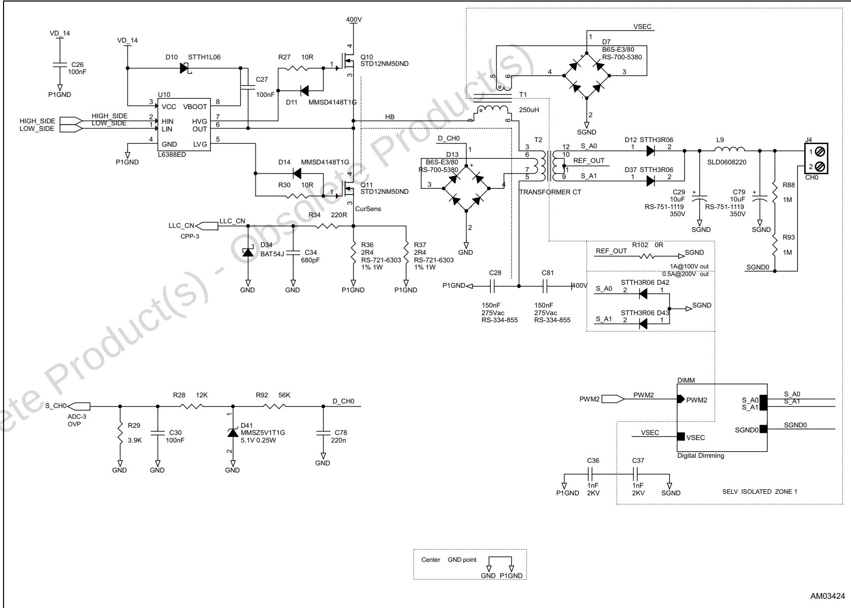
Figure 4. PSR-ZVS demonstration board schematic - PSR-ZVS stage
