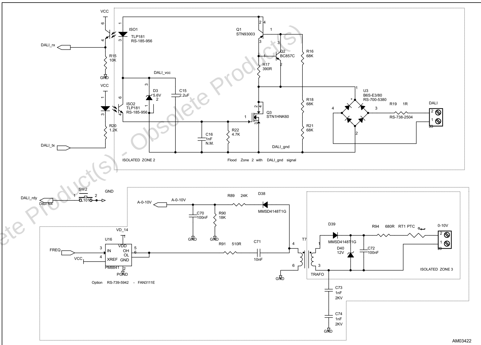
Figure 7. PSR-ZVS demonstration board schematic - DALI and 0 - 10 interfaces
