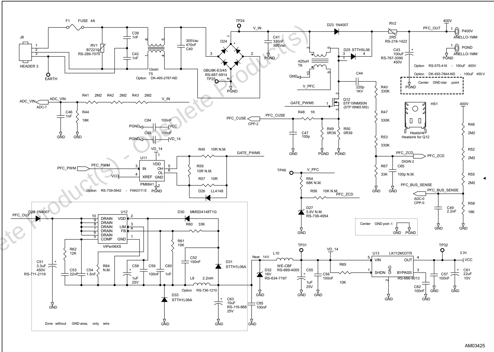
Figure 3. PSR-ZVS demonstration board schematic - PFC and DC/DC zone
