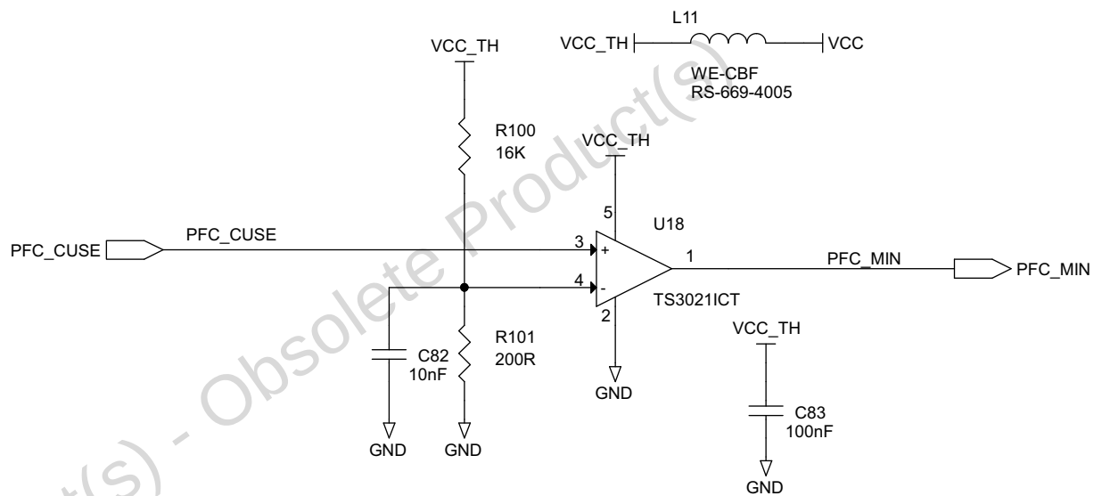
Figure 6. PSR-ZVS demonstration board schematic - THD optimizer
