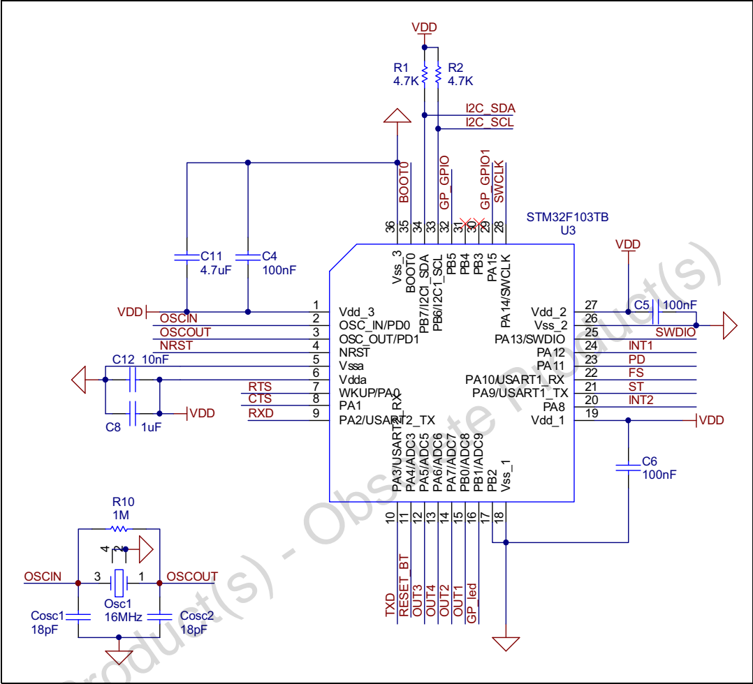
Figure 3. Microcontroller
