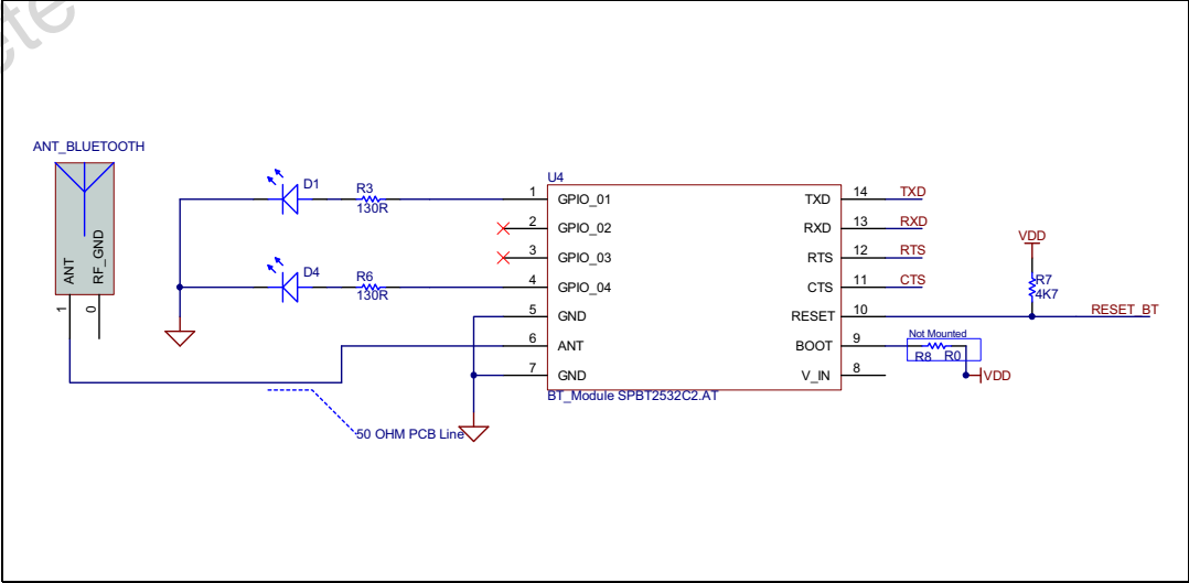
Figure 4. Bluetooth module
