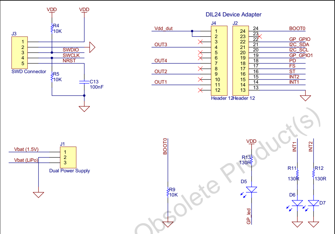
Figure 2. Connectors
