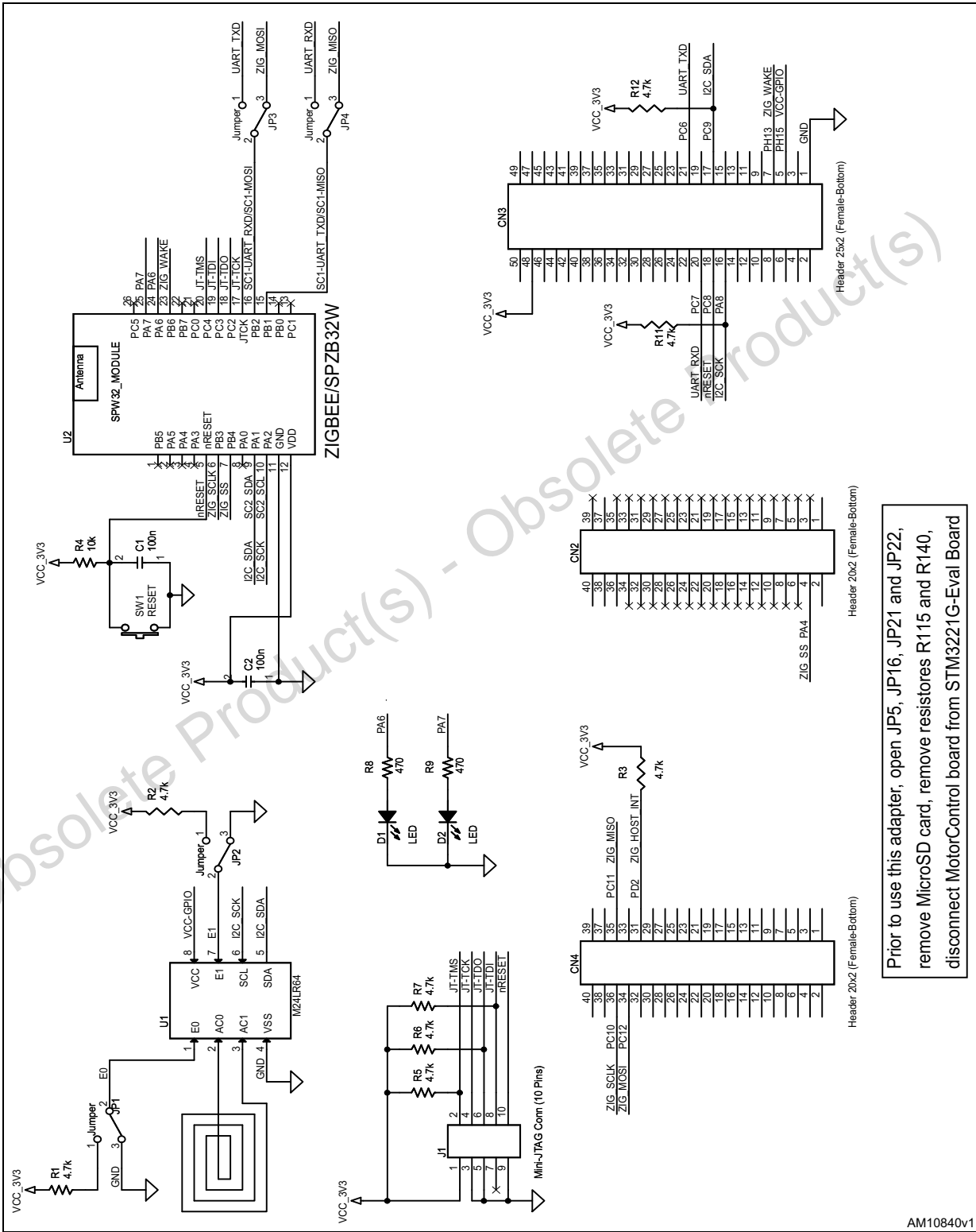
Figure 1. Circuit schematic
