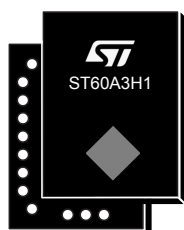
VFBGA23 AiP LP (2.9 mm x 4.1 mm x 0.8 mm)
