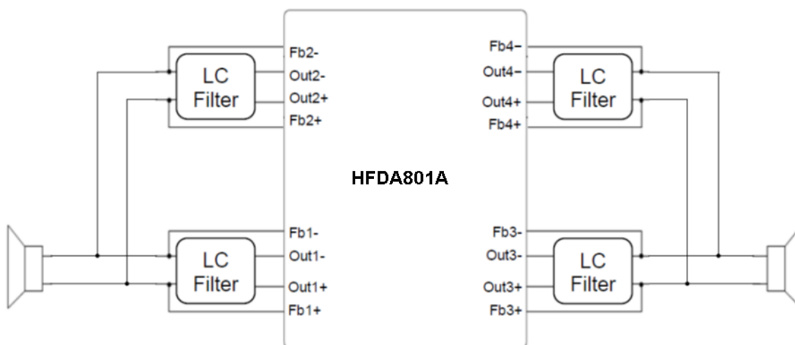
Figure 3. Parallel mode configuration
