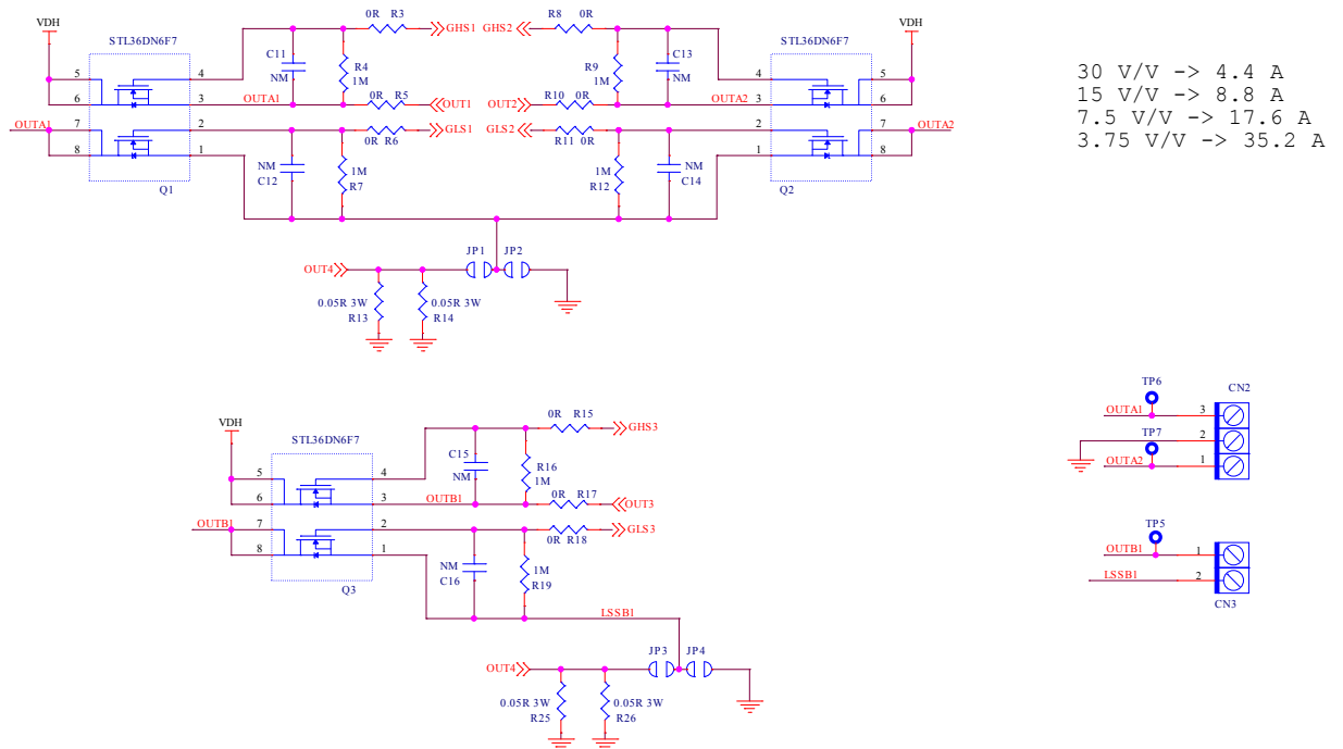
Figure 2. Schematic board 2
