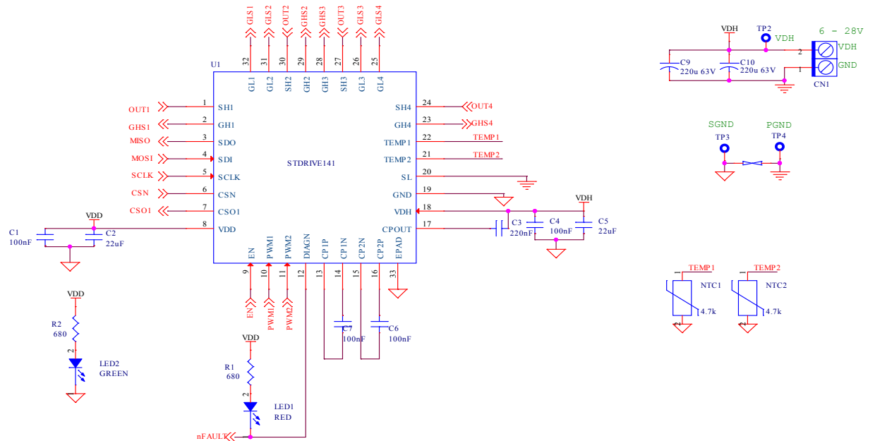
Figure 1. Schematic board 1
