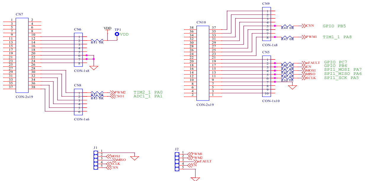
Figure 3. Schematic board 3
