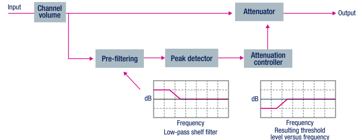
Figure 3: EqDRC block diagram
