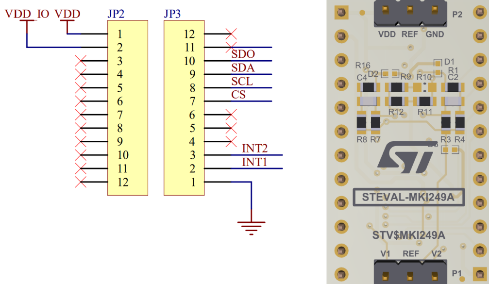
Figure 15. STEVAL-MKI249A DIL24 adapter board pinout (ST1VAFE6AX)
