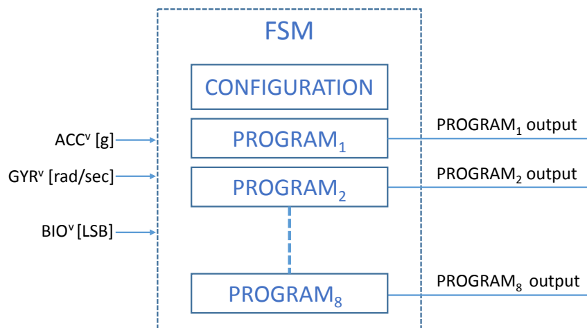
Figure 4. FSM block
