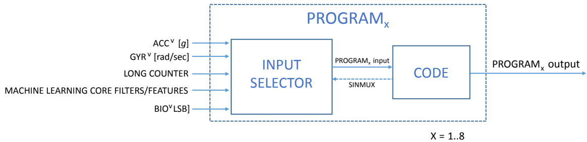
Figure 5. Program block
