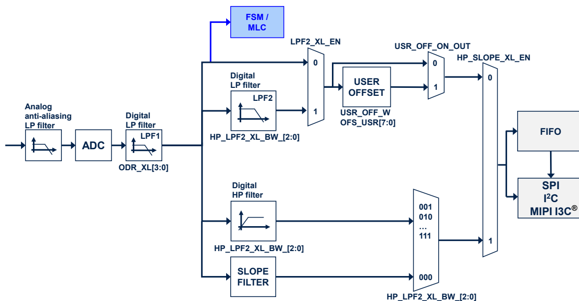
Figure 6. FSM inputs (accelerometer)
