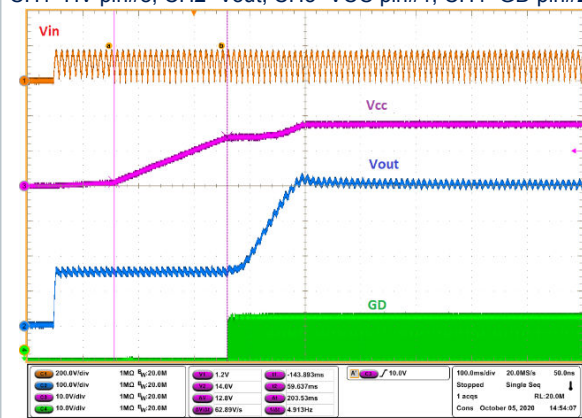
Figure 17. Start-up voltage waveforms (115Vac)
