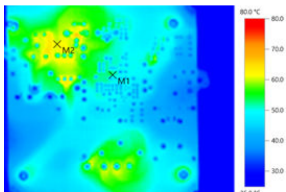
Figure 64. Thermal measurements at 115Vac - full load (bottom side)
