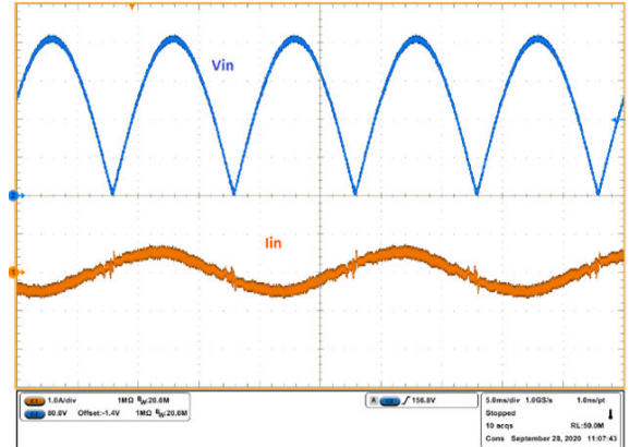
Figure 28. Steady-state - input current at 20% load (230Vac)
