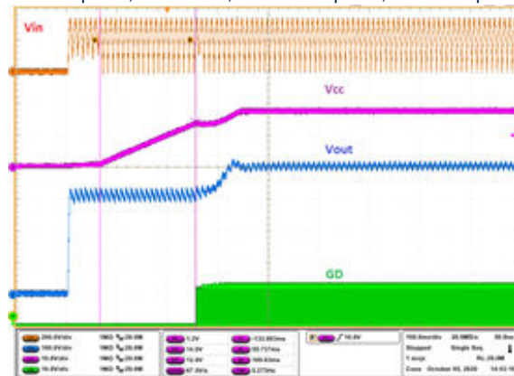
Figure 18. Start-up voltage waveforms (230Vac)
