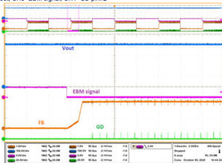
Figure 52. External burst mode - exit
