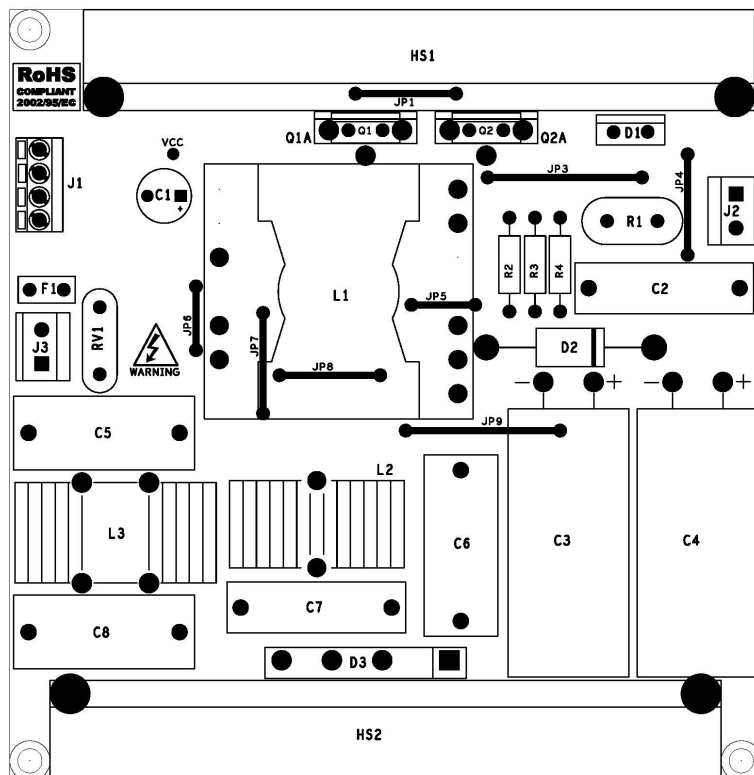
Figure 5. EVL4985-350W PCB layout (top side)
