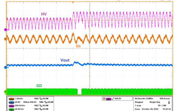
Figure 62. Line variation – “High-line” and 10% load (265Vac to 175Vac)
