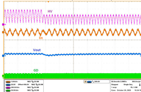
Figure 61. Line variation – “High-line” and 10% load (175Vac to 265Vac)
