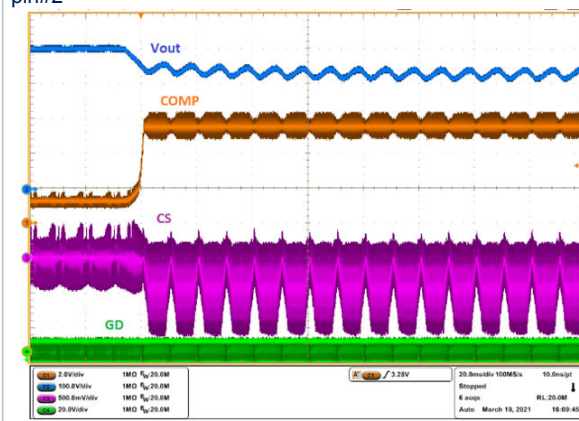
Figure 53. Output overload (a)
