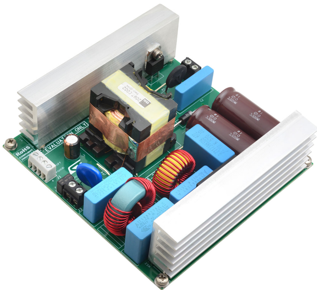
Figure 1. EVL4985-350W demonstration board
