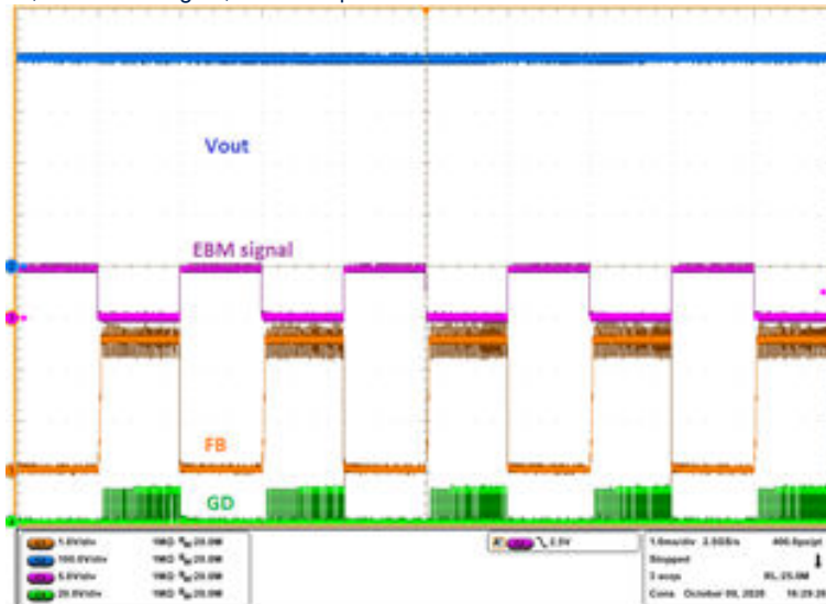
Figure 51. External burst mode
