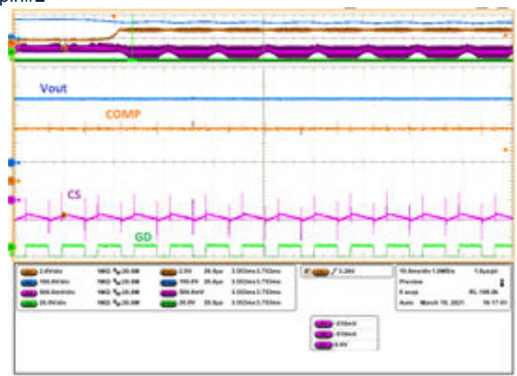
Figure 54. Output overload (b)
