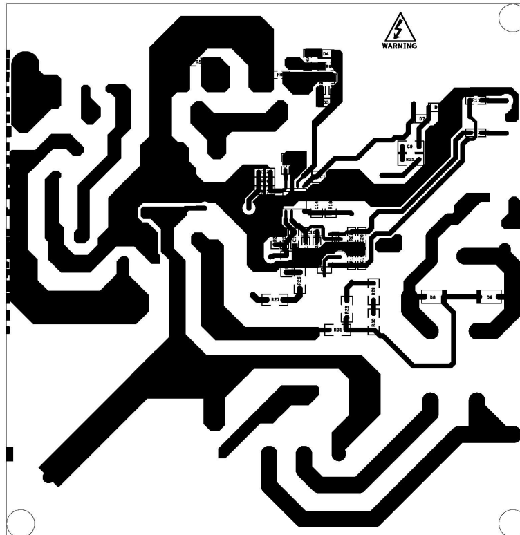
Figure 6. EVL4985-350W PCB layout (bottom side)
