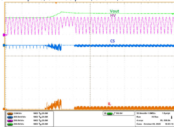
Figure 22. Start-up at light load (230Vac)
