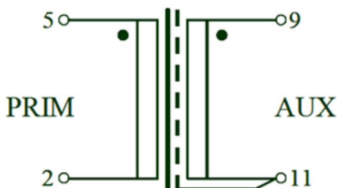
Figure 69. Boost inductor – electrical diagram
