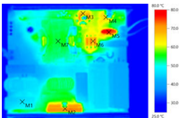
Figure 63. Thermal measurements at 115Vac - full load (top side)
