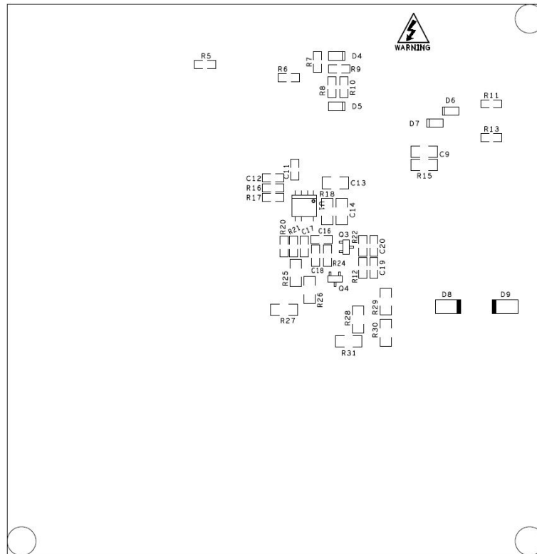
Figure 4. EVL4985-350W PCB component placement (bottom side)
