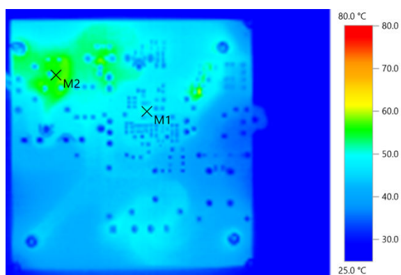
Figure 66. Thermal measurements at 230Vac - full load (bottom side)
