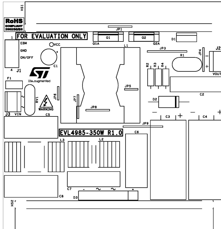
Figure 3. EVL4985-350W PCB component placement (top side)
