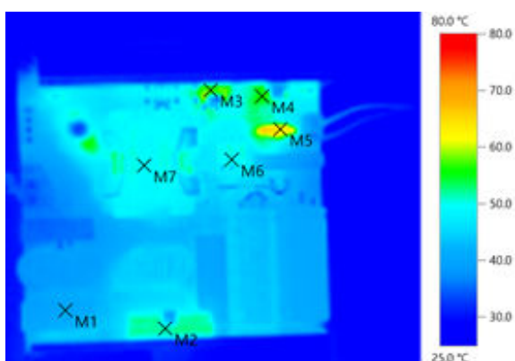
Figure 65. Thermal measurements at 230Vac - full load (top side)
