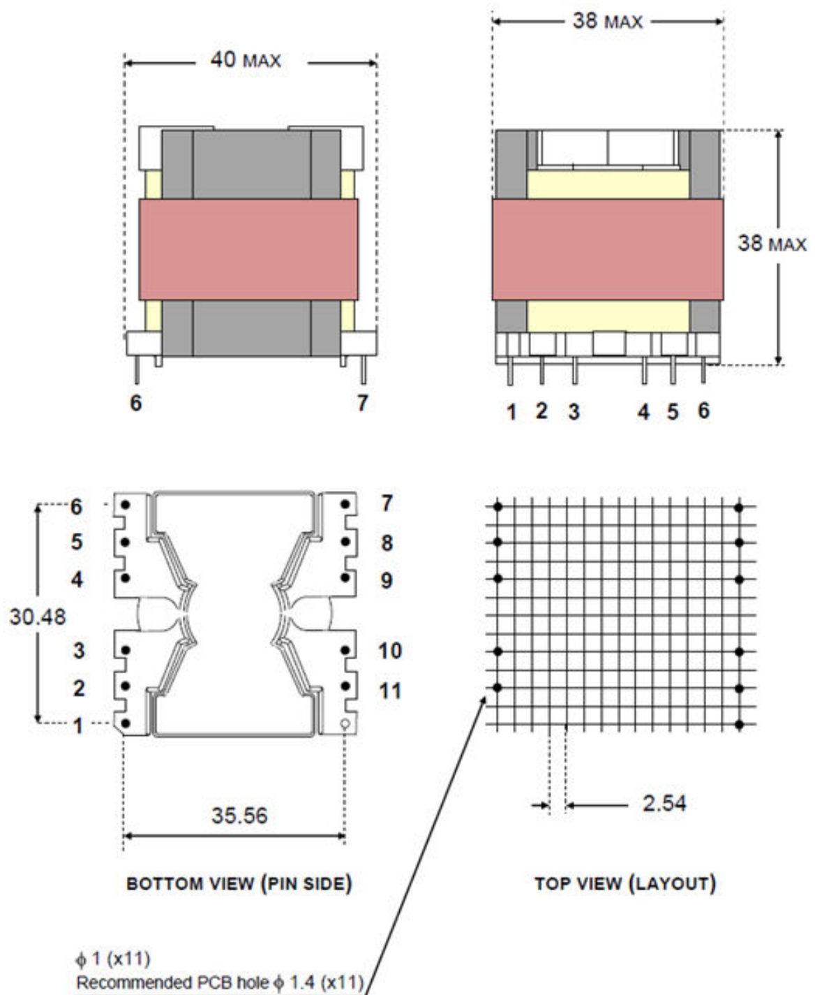
Figure 70. Boost inductor – mechanical drawing
