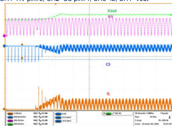
Figure 20. Start-up at full load (230Vac)
