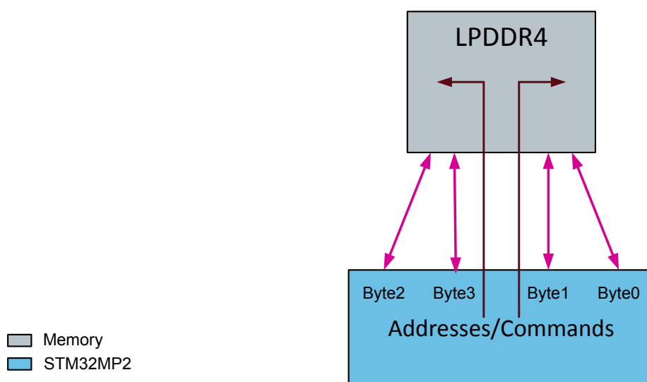
Figure 1. 32-bit LPDDR4 interface
