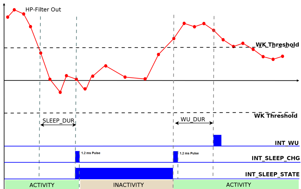
Figure 17. Activity/inactivity recognition (using the HP filter)
