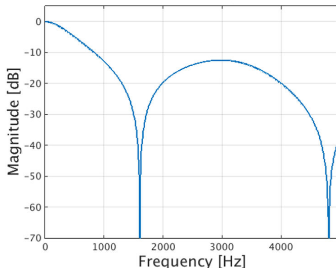
Figure 5. LPF1 - high-performance mode, ODR = 1600 Hz, BW = 400 Hz
