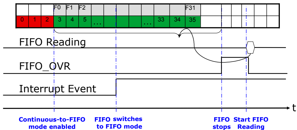
Figure 21. Continuous-to-FIFO mode: interrupt latched and nonlatched
