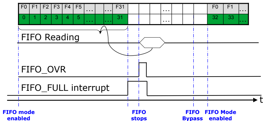
Figure 18. FIFO mode behavior
