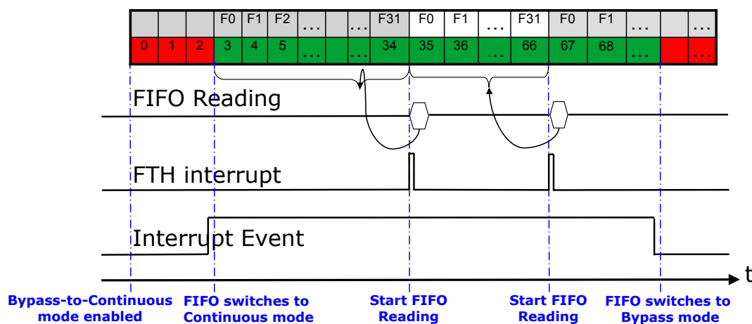
Figure 20. Bypass-to-continuous mode
