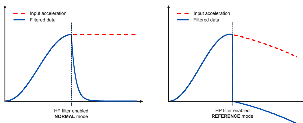
Figure 4. High-pass filter in normal and reference mode
