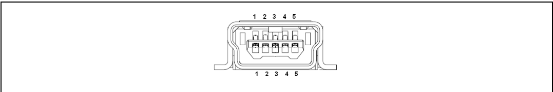
Figure 19. USB mini-B connector (CN1)
