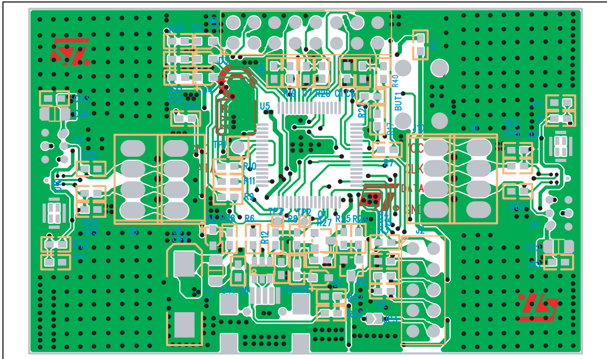
Figure 11. Board layout - bottom view
