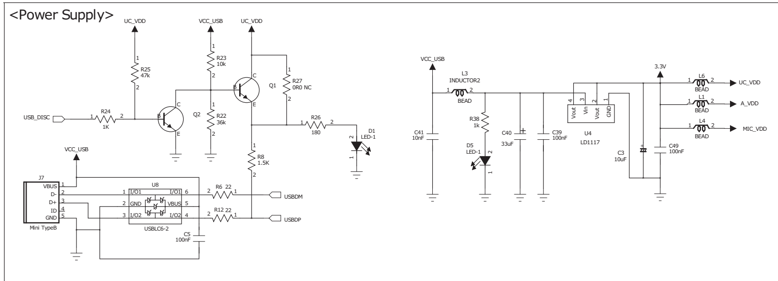
Figure 8. Board schematic (power supply and JTAG connector)
