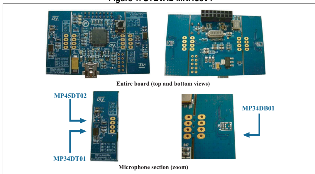
Figure 1. STEVAL-MKI138V1
