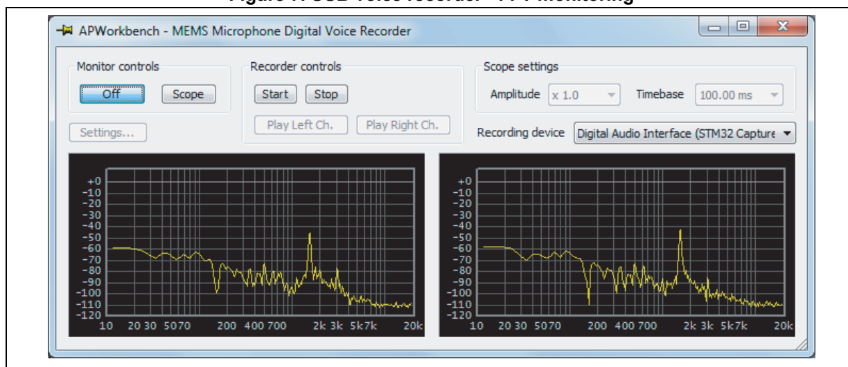
Figure 7. USB voice recorder - FFT monitoring
