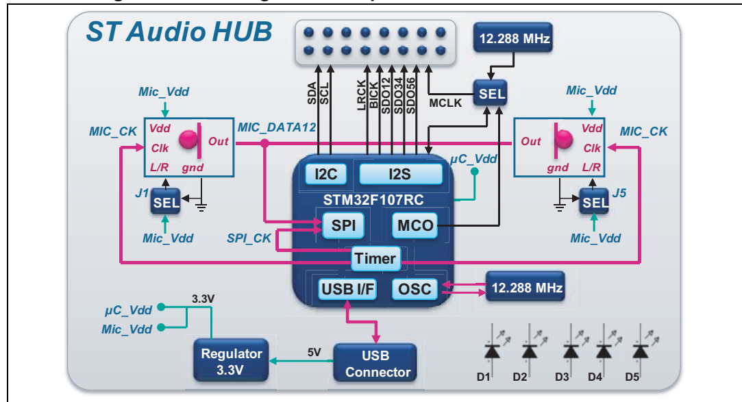
Figure 2. Block diagram - microphone USB demonstration board
