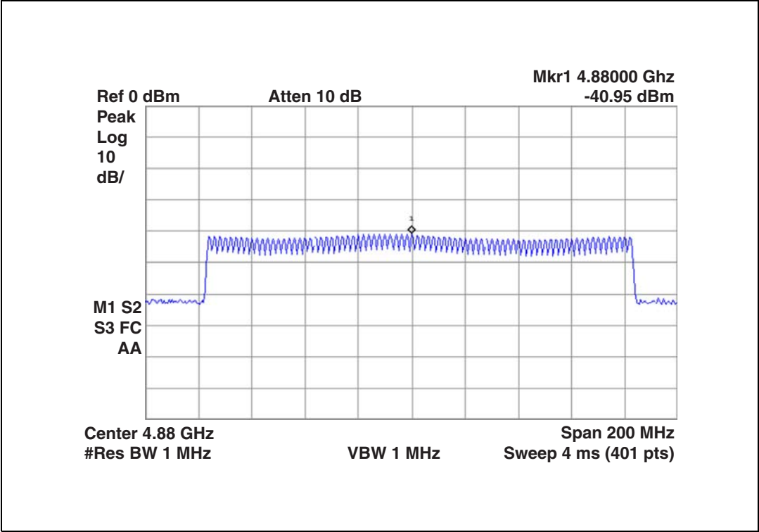
Figure 10. Second harmonic
