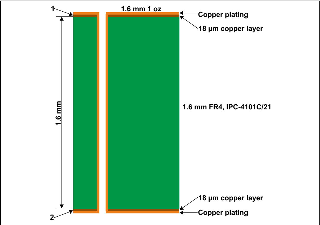
Figure 24. PCB stack-up recommendation
