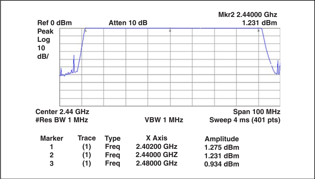
Figure 9. Output power carrier
