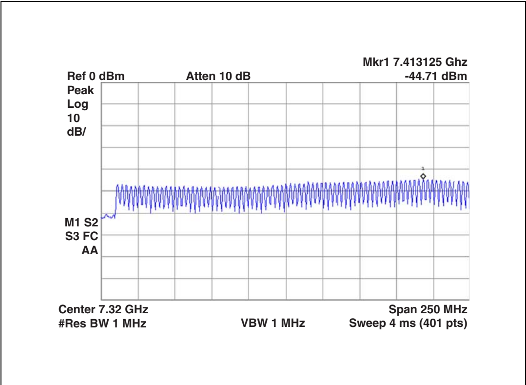
Figure 11. Third harmonic
