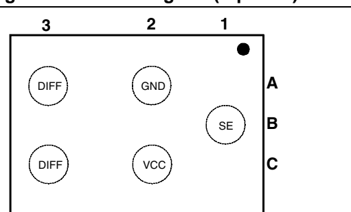
Figure 2. Pin out diagram (top view)
