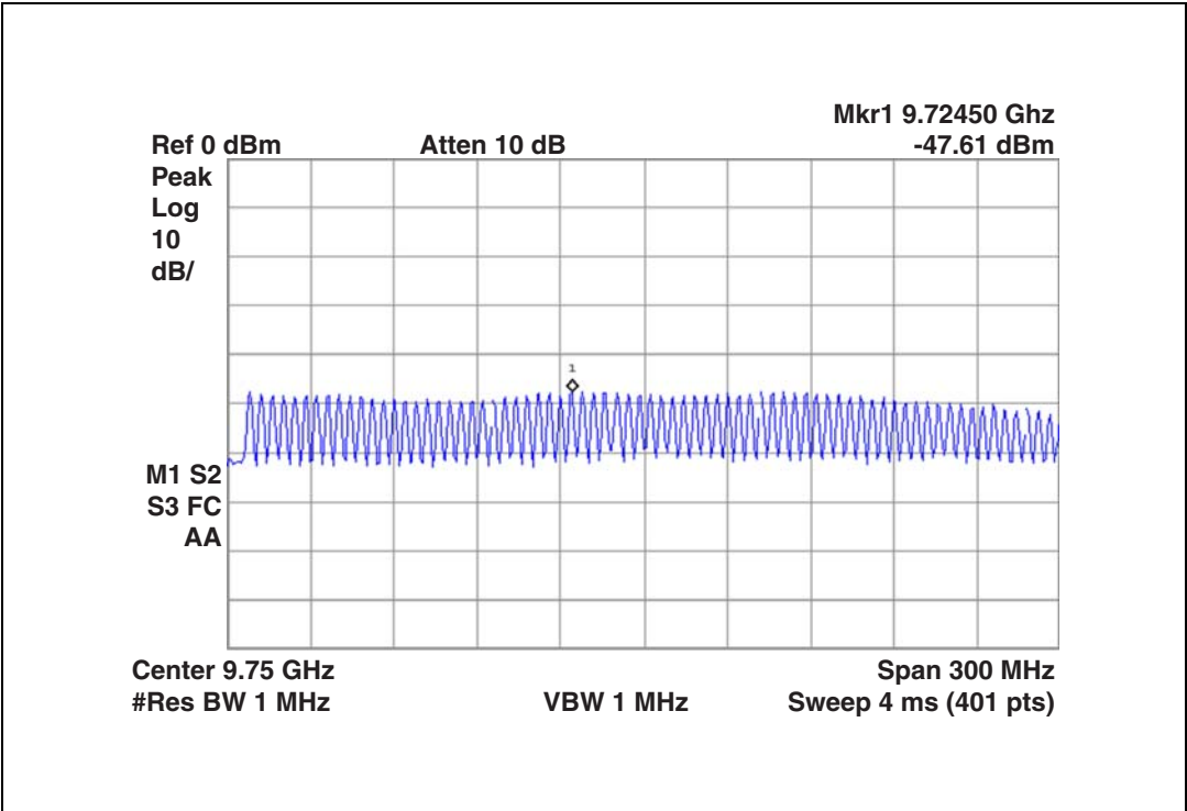
Figure 12. Fourth harmonic
