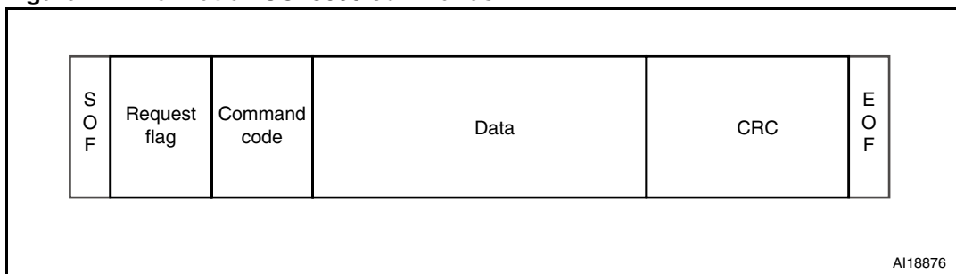
Figure 4. Format of ISO15693 commands
