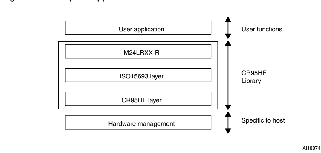
Figure 2. Example of application architecture
