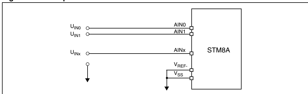
Figure 11. Multiple channel measurement
