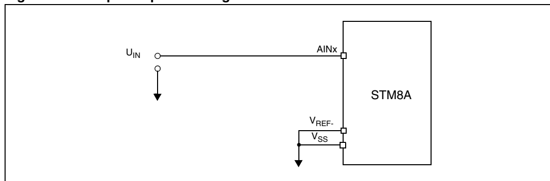
Figure 6. Simple unipolar DC signal measurement
