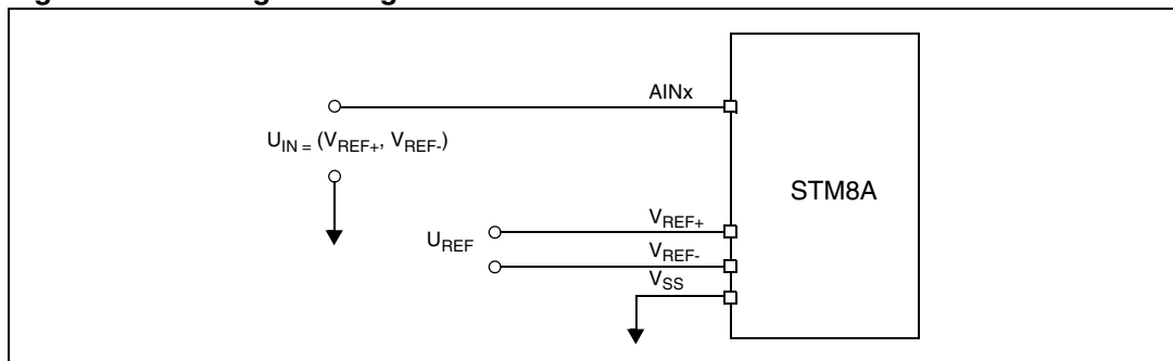
Figure 10. Analog zooming
