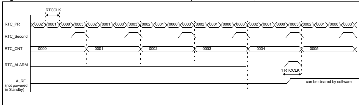
Figure 4. RTC second and alarm waveform example with PR=0003, ALARM=00004
