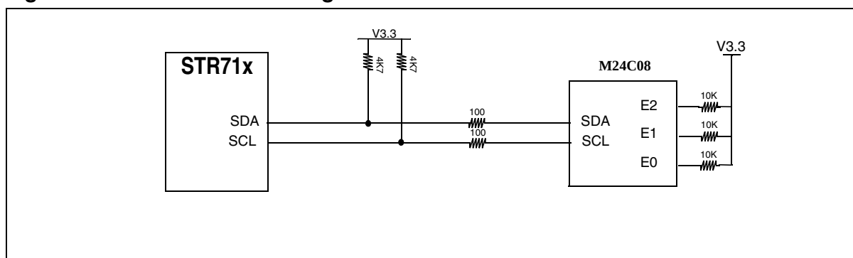
Figure 1. STR71x/M24C08 configuration
