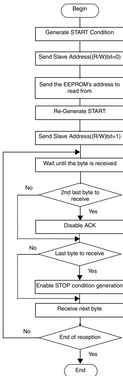
Figure 3. Read Operation Flowchart
