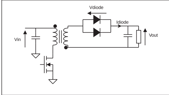
Fig. 4: Topology of a flyback converter.
