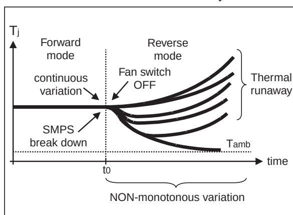
Fig. 6: Example of junction temperature variation in non-constant thermal resistance system
