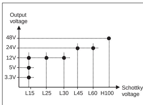
Fig. 2: Typical Schottky used as OR-ing function on common voltage outputs
