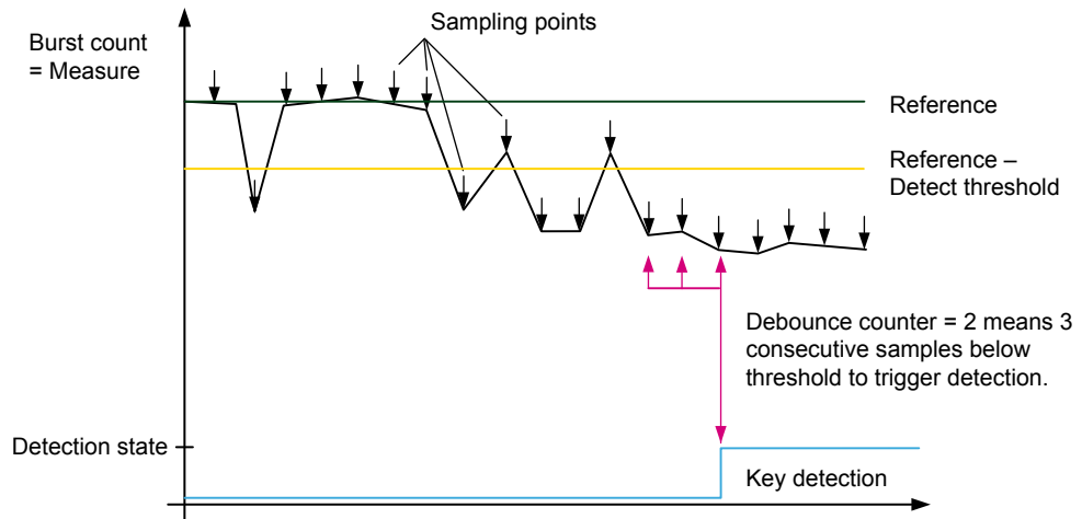
Figure 9. Debouncing example
