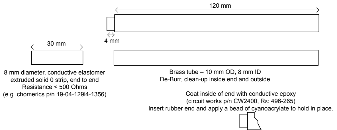
Figure 5. Recommended standard finger
